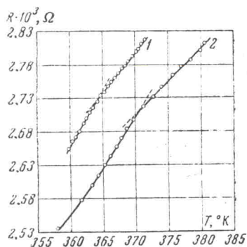
FIG. 2. Temperature dependence of electric resistance: 1 – at atmospheric pressure ( T_N = 364.6^\circ ), 2 – at T = 8850 kg/cm 2 ( T_N = 370.7^\circ ).
